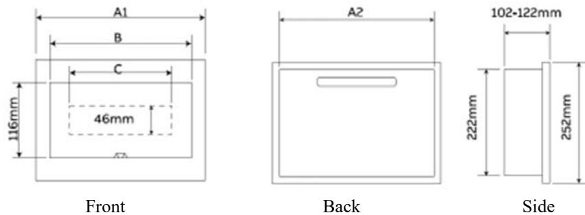
Dimension drawings of surface mounted distribution box
