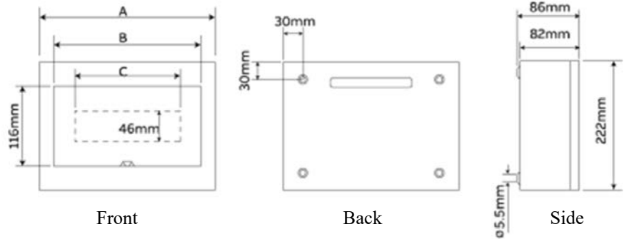
Dimension drawings of surface mounted distribution box
