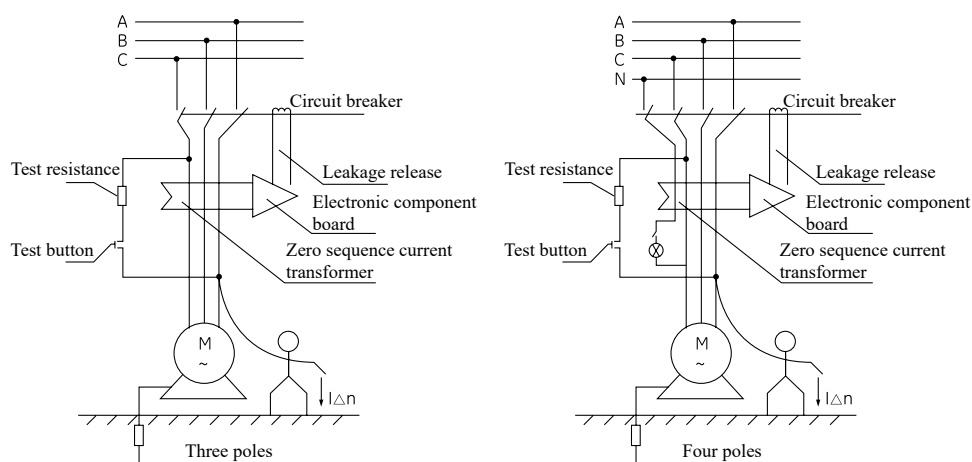
Fig. 1 Working principle
