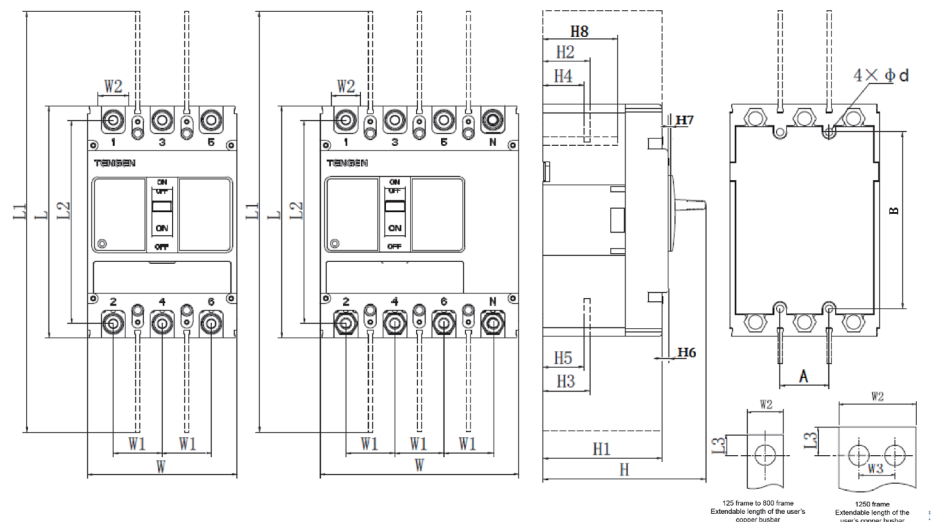
Fig. 1 Outline dimensions and installation dimensions of TGM1E
