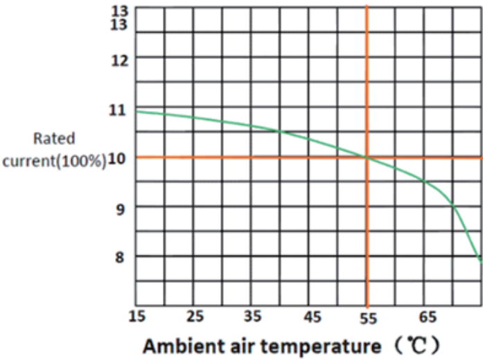
Temperature compensation curve of 500-800A
