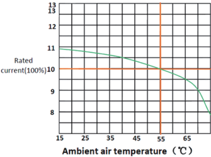
Temperature compensation curve of 1000-1250A
