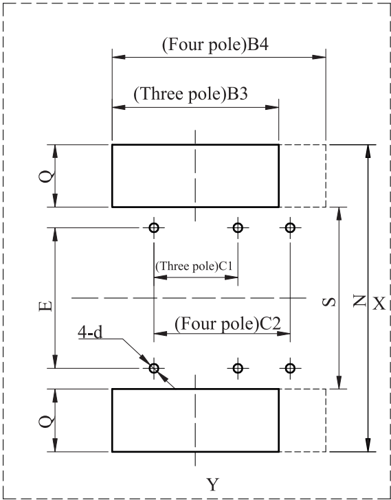
12.2 Opening size of mounting plate (unit: mm)
