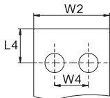
Copper bar insertion length for 1250/1600 shell frame
