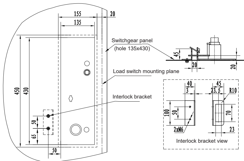
6.3 Cabinet door hole and interlock installation diagram (with right console installed at front side)
